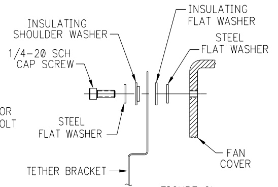
FIGURE 2b FAN COVER MOUNT WITH THREADED HOLE
