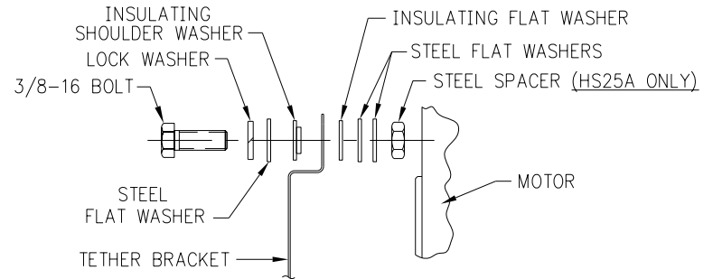
FIGURE 3 MOTOR HOUSING MOUNT NEMA 4.50 C-FACE
