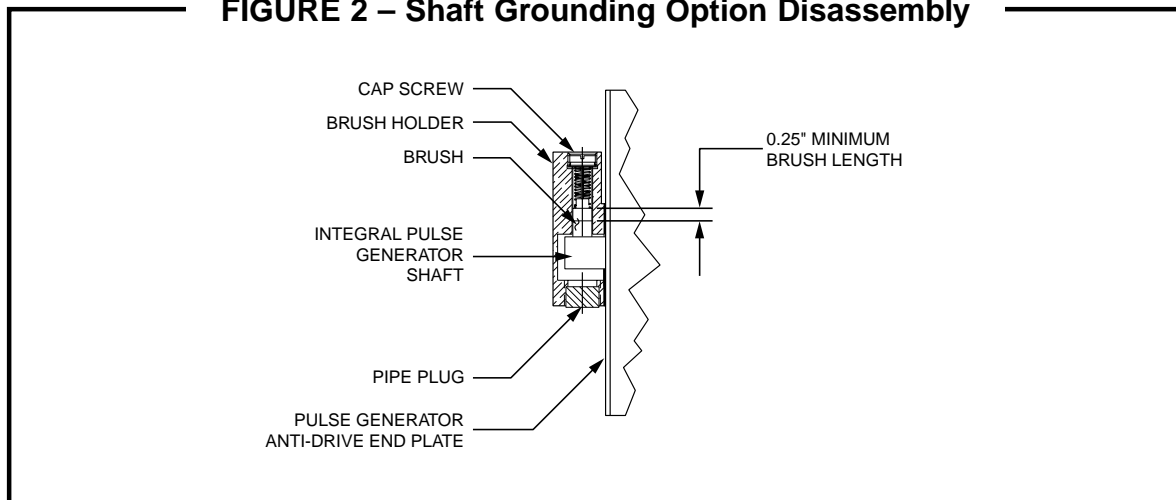
FIGURE 2 – Shaft Grounding Option Disassembly
